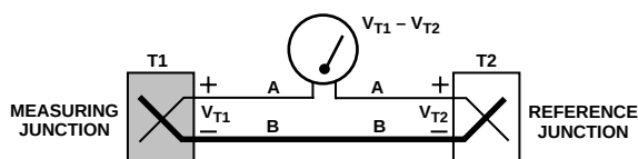
Figure 1a. Thermocouple Loop
