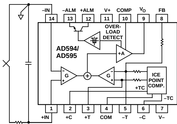
Figure 4. Input Filtering
