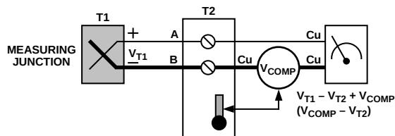
Figure 1d. Cold Junction Compensation
