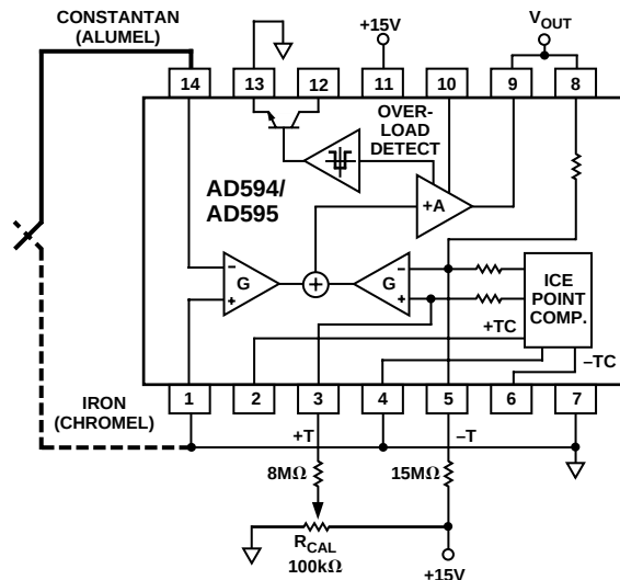
Figure 5. Optional Calibration
